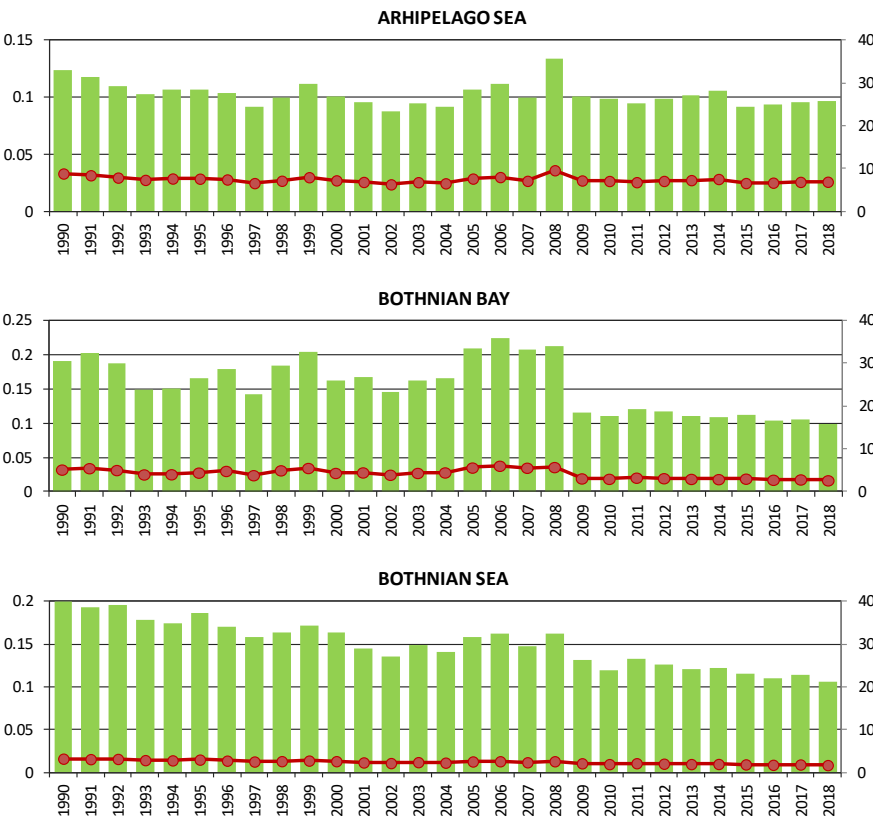
Figure 2. Time-series of computed total annual atmospheric deposition of B(a)P to nine sub-basins of the Baltic Sea for the period 1990-2018 in tonnes/year as bars (left axis) and total deposition fluxes in g/m 2 /year as lines (right axis).
